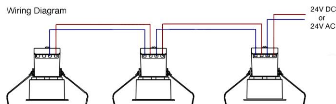
Wiring Diagram
