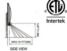
Wall Mount sensor Detection Range
